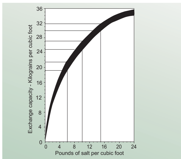
Fig. 1 Exchange capacity vs. regeneration level Sodium form C-800 LT Cation Resin
